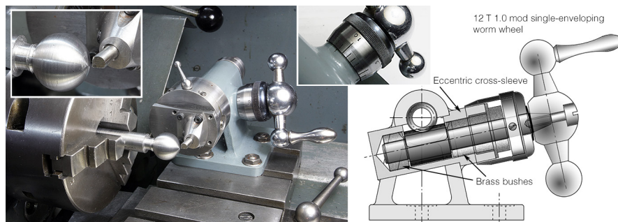
Figure 2.25: The author's spherical turning attachment
