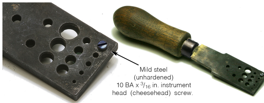
Figure 2.3: Heat bluing plate for screws
