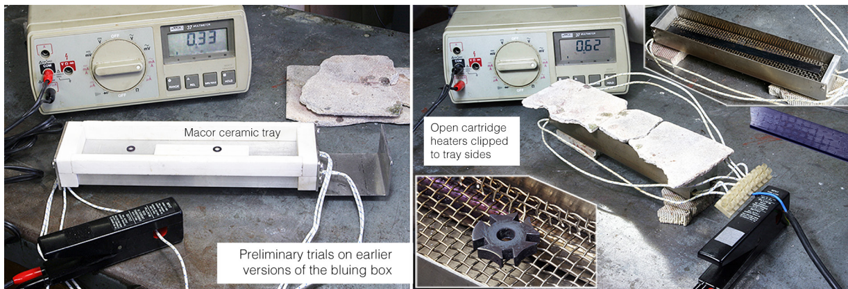
Figure 2.14: Trials on earlier Versions of the bluing box
