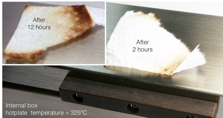
Figure 2.8: The results of the fire test
