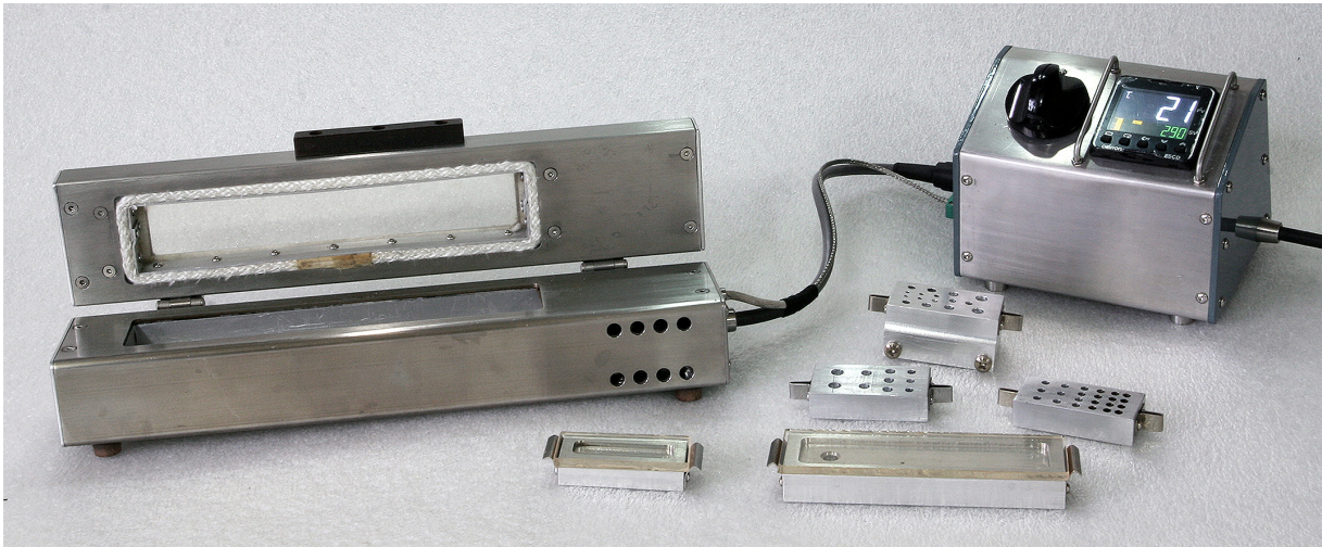
Figure 2.6: Version 4 of the author's PID-controlled bluing box and accessories
