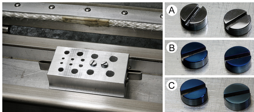
Figure 2.16: Trials on bluing screws:
