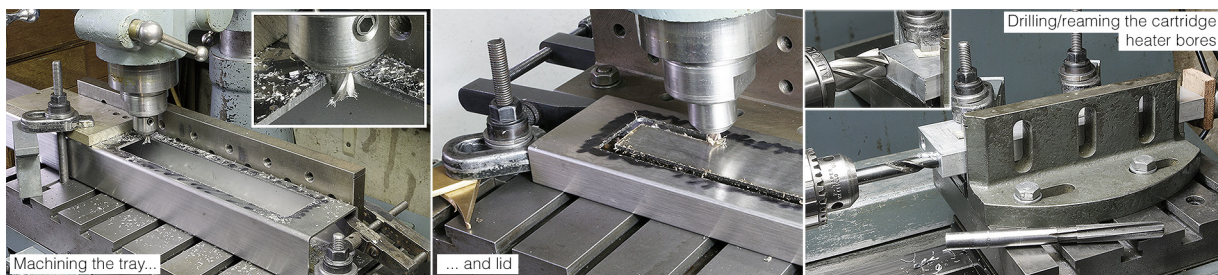
Figure 2.11: Cutting the openings in the stainless steel RHS, and (right) drilling the hotplate for the cartridge heaters
