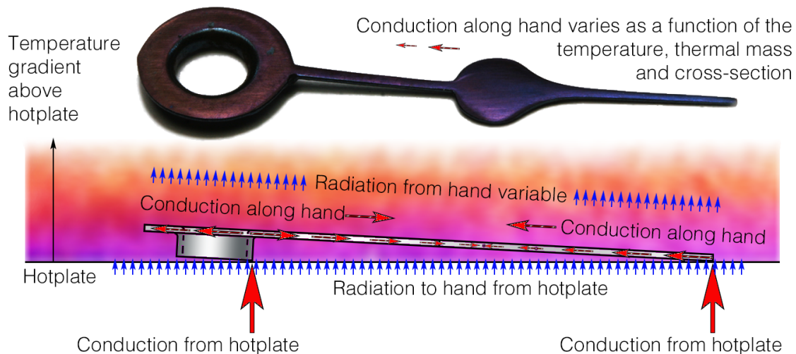
Figure 2.20: Heat transfer mechanisms from hotplate to a clock hand
