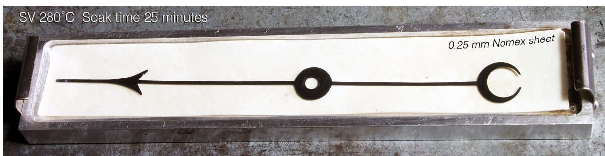
Figure 2.24: A successful trial on a barometer hand using Nomex paper
