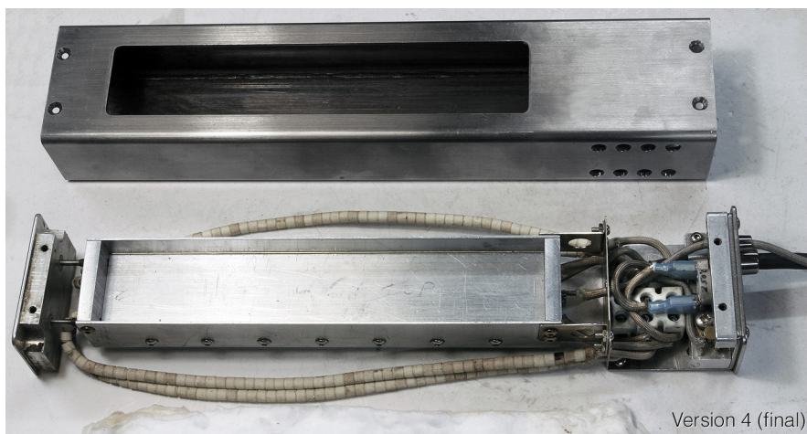
Figure 2.9: The bluing tray construction
