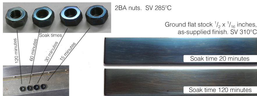
Figure 2.15: Trials on earlier Versions of the bluing box
