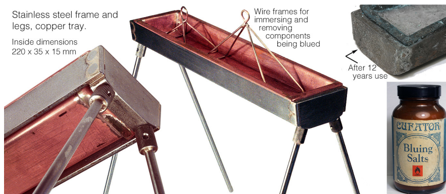
Figure 2.4: Bluing salts tray
