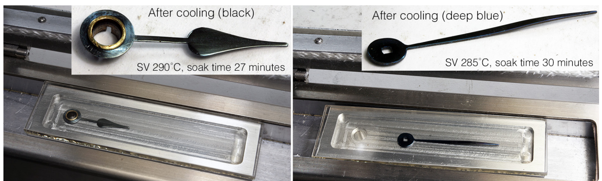
Figure 2.23: Further trial results on bluing clock hands
