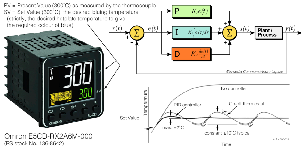
Figure 2.7: The PID controller and an outline of its system diagram (top right) and a comparison of alternative methods of control (bottom right)
