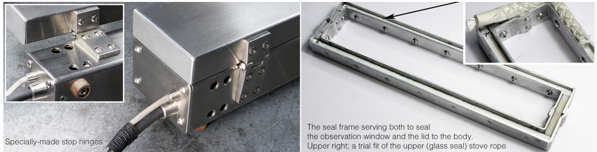
Figure 2.12: Further details of the bluing box
