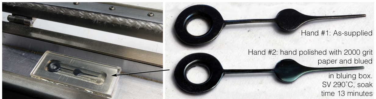
Figure 2.22: Comparison of a professionally blued hand (upper right) with one blued in the bluing box (lower right)
