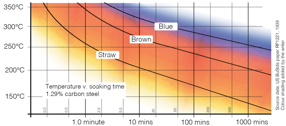
Figure 2.5: Heat colouring chart showing dependency on both temperature and time
